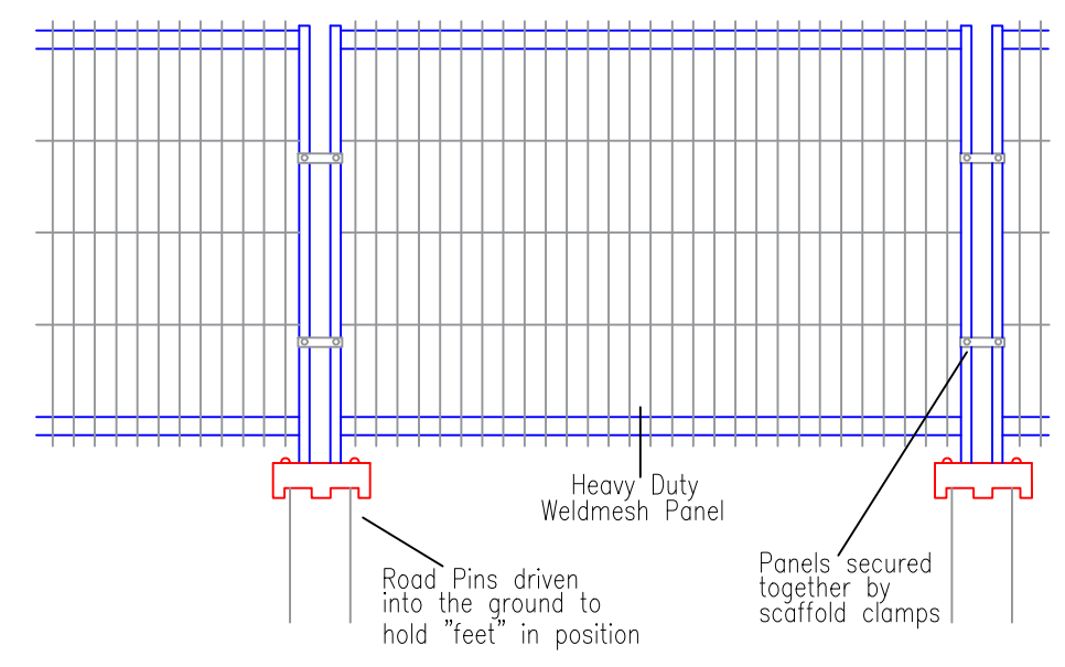
FIGURE 3, HERAS WELDMESH PANEL TREE PROTECTION BARRIER TO BS5837:2012
