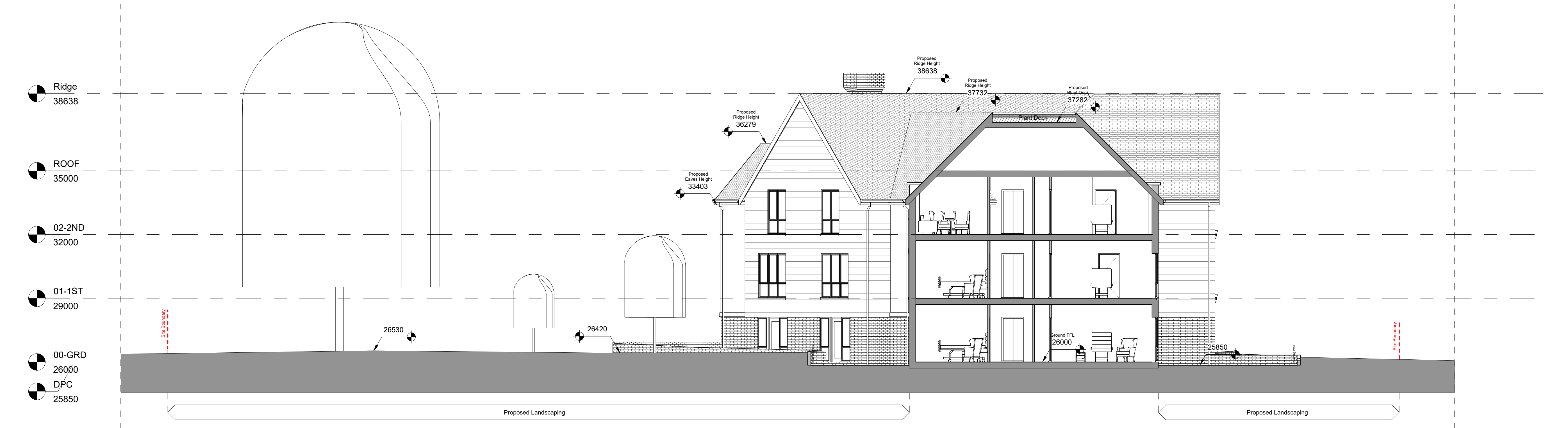
2 Proposed Site Section B-B 1 : 100
