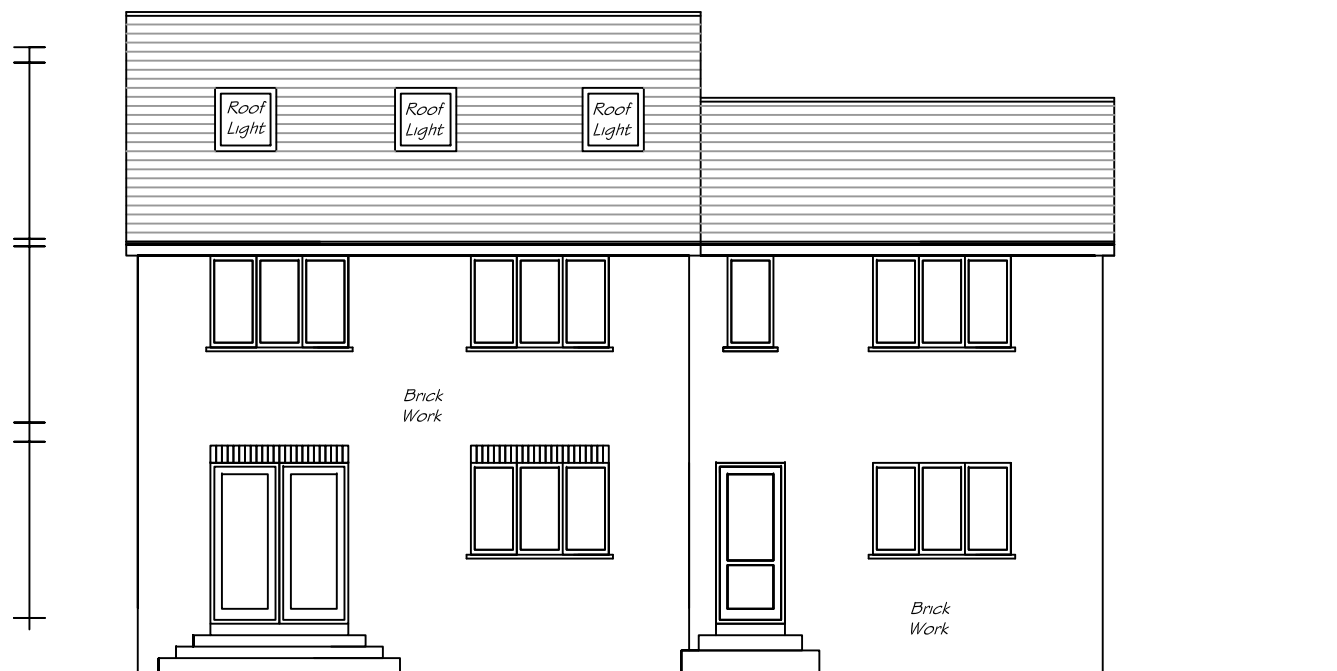
PROPOSED REAR ELEVATION B.
