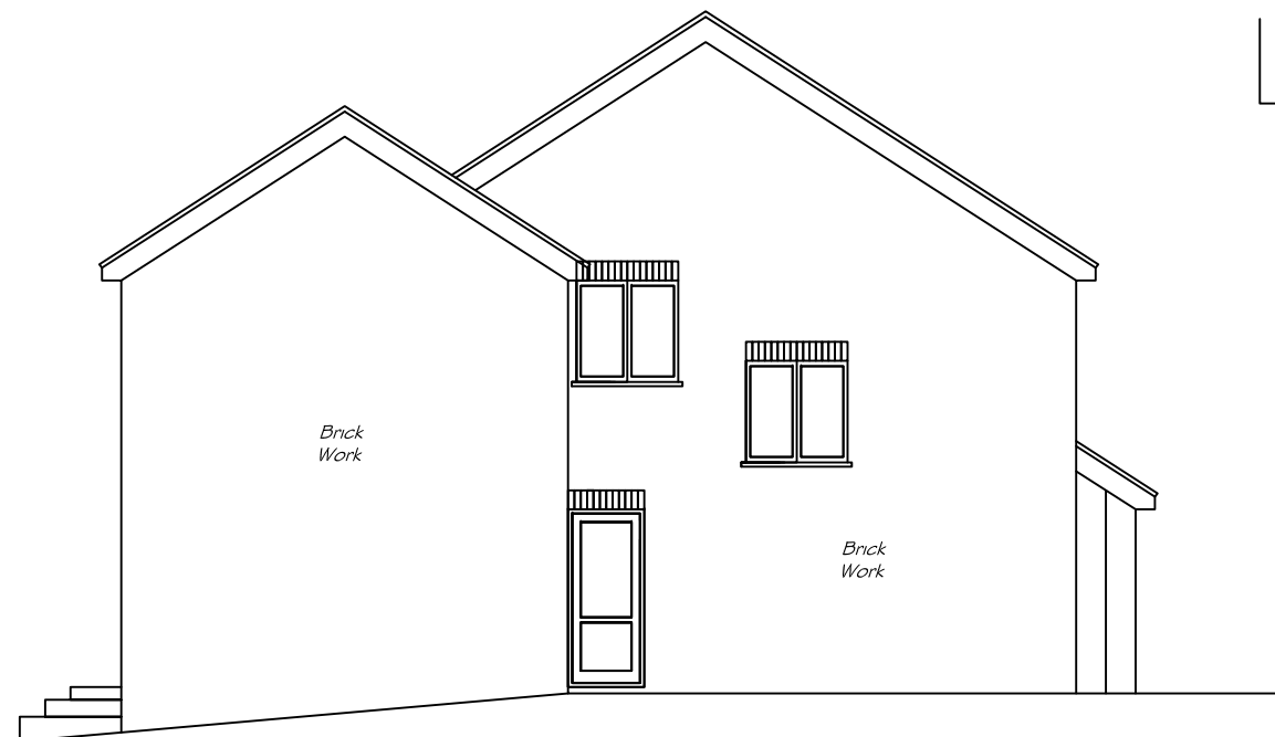
PROPOSED SIDE ELEVATION B.
