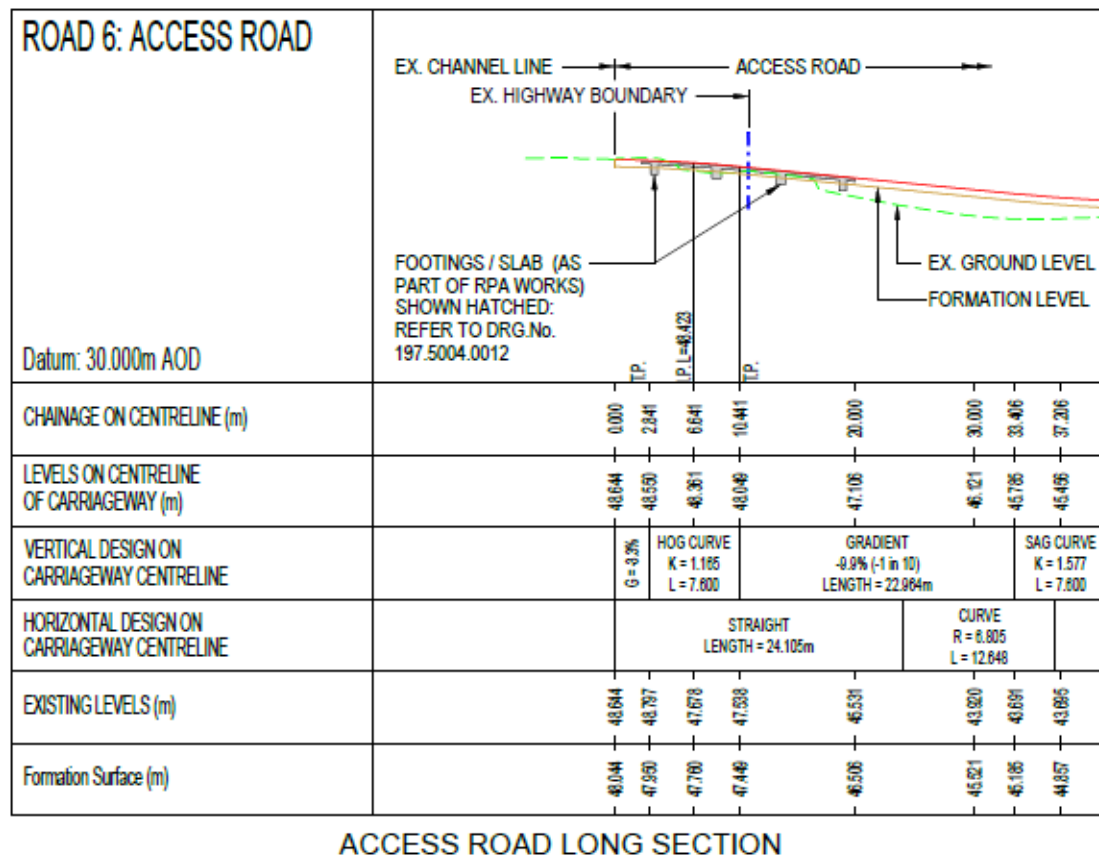
Figure 2: Supplied long section drawing of strip foundation design.
