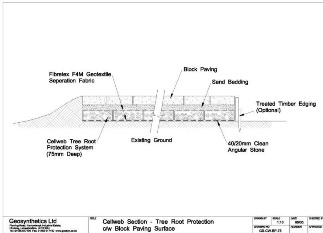
Figure 4 Cellular system profile
