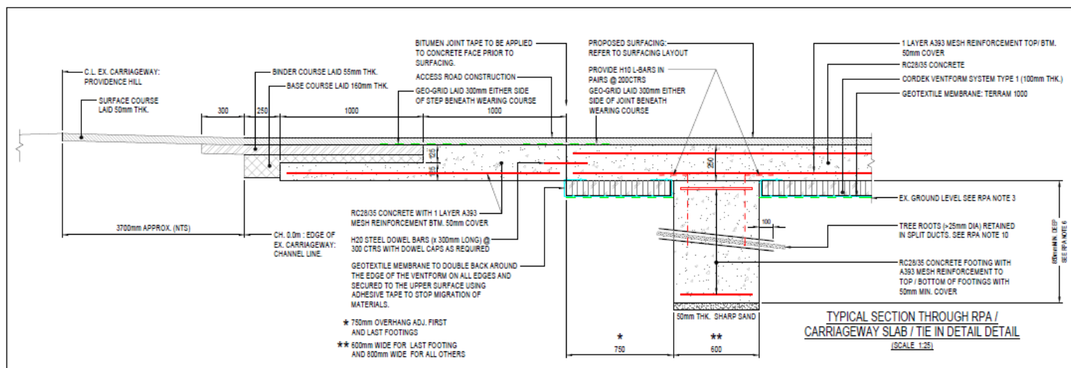
Figure 3: Further supplied drawing from Paul Basham Associates.
