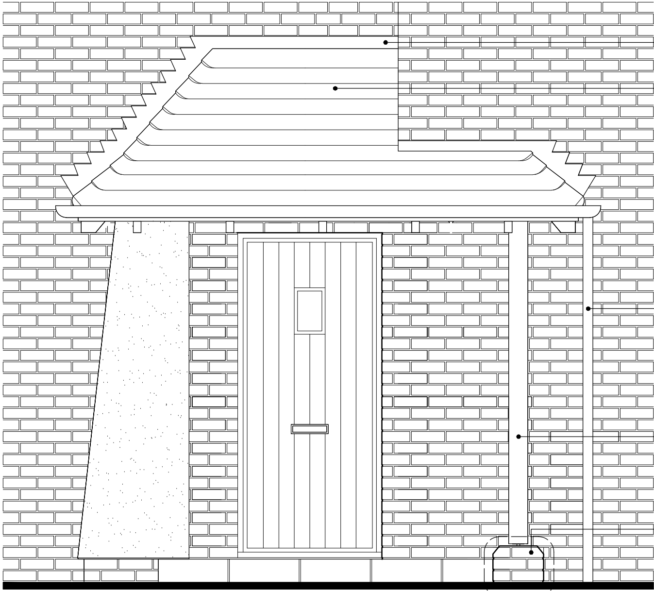
FRONT ELEVATION (SCALE 1:20)
