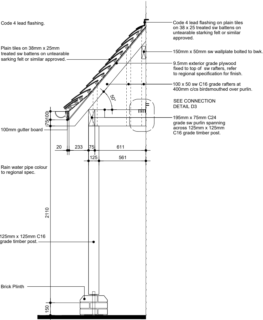
SECTION THRU' (1:20)
