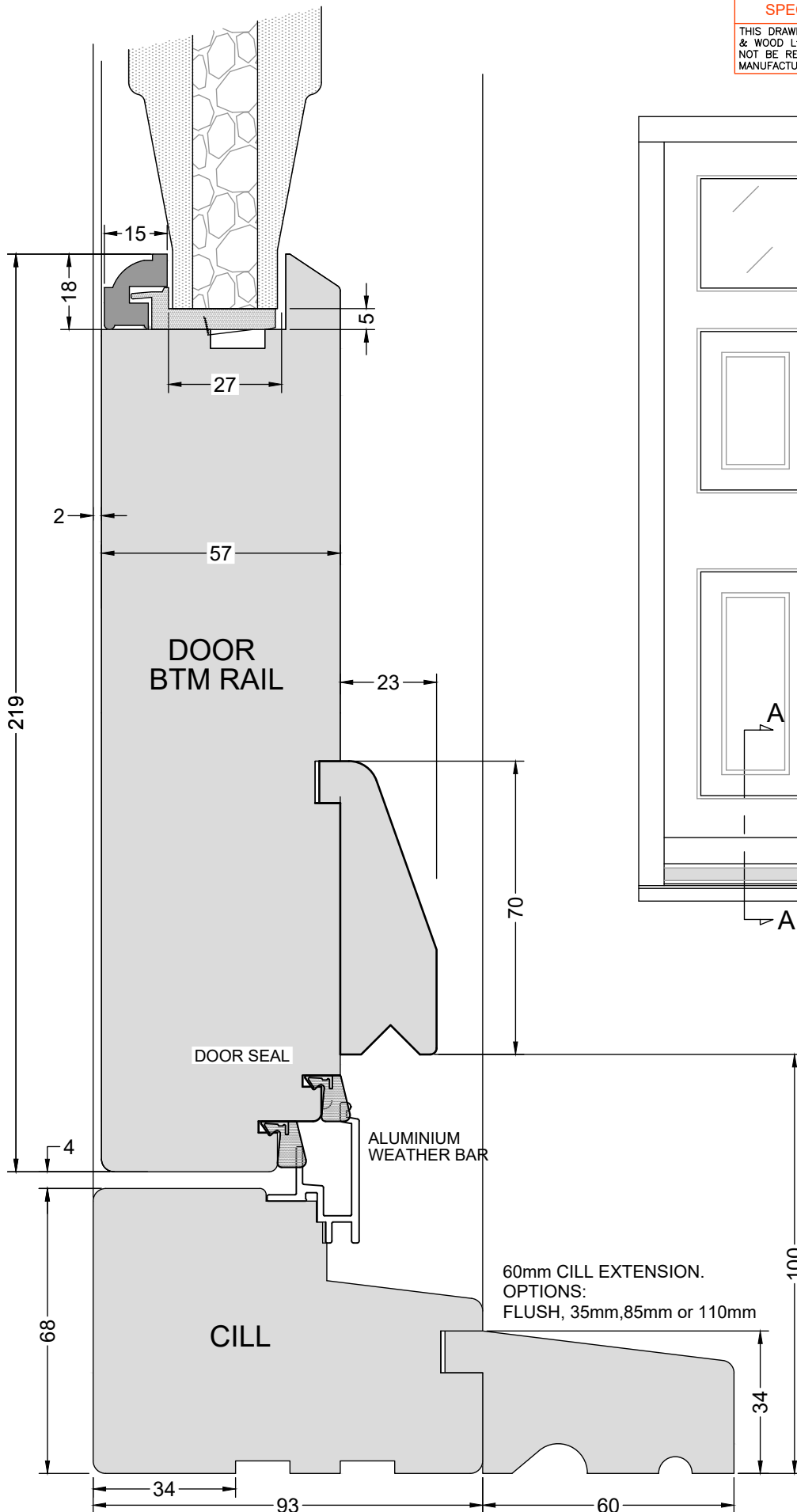
CILL SECTION A-A
