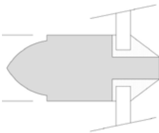
PROFILE AVAILABLE IN 18MM GLASS SHOWN AS 4MM
