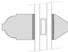
PROFILE AVAILABLE IN 18MM OR 22MM GLASS SHOWN AS 14MM DOUBLE GLAZED UNIT
