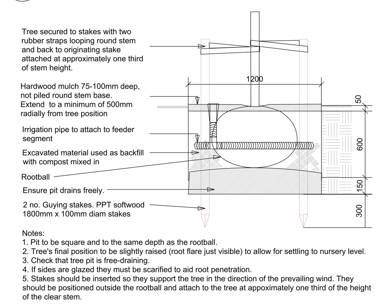
100 02 Proposed Tree Pit Detail - where tree is located in soft landscape Scale 1:20 @ A1
