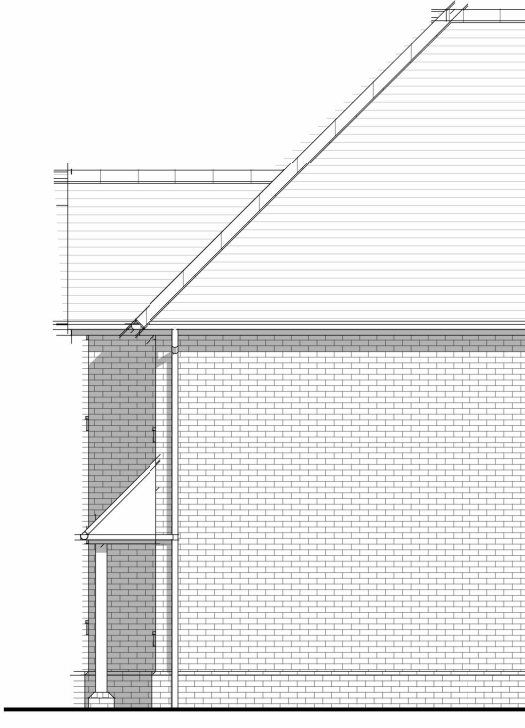
Existing Side Elevation (West) 1 : 100
