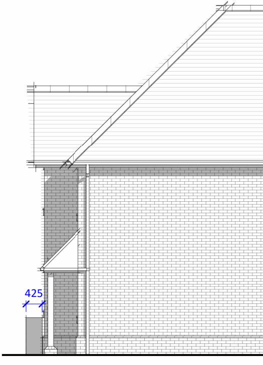
Proposed Side Elevation (West) 1 : 100
