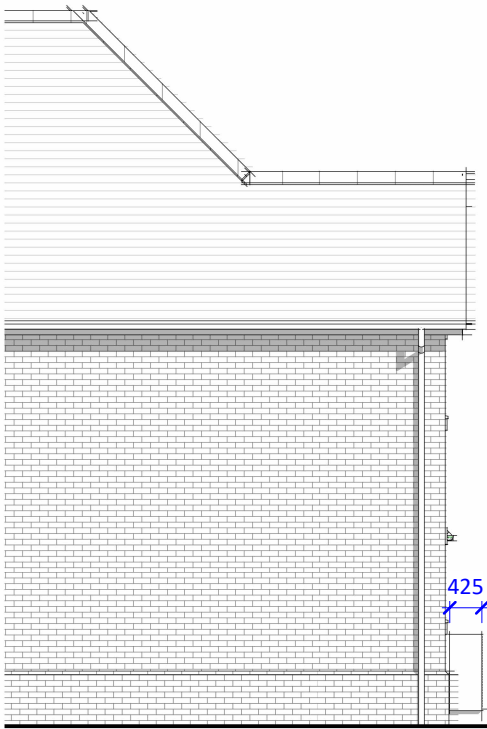
Proposed Side Elevation (East) 1 : 100
