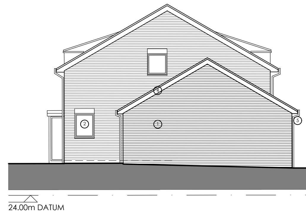
SIDE, NORTH ELEVATION
