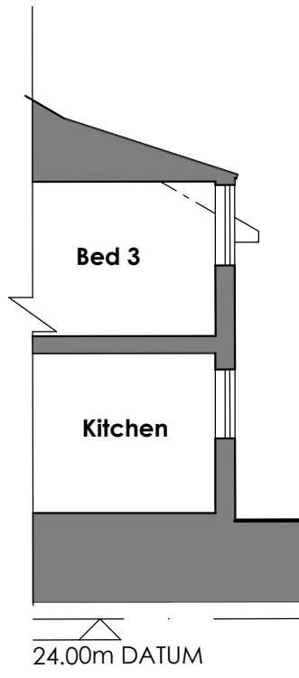
SECTION B-B
