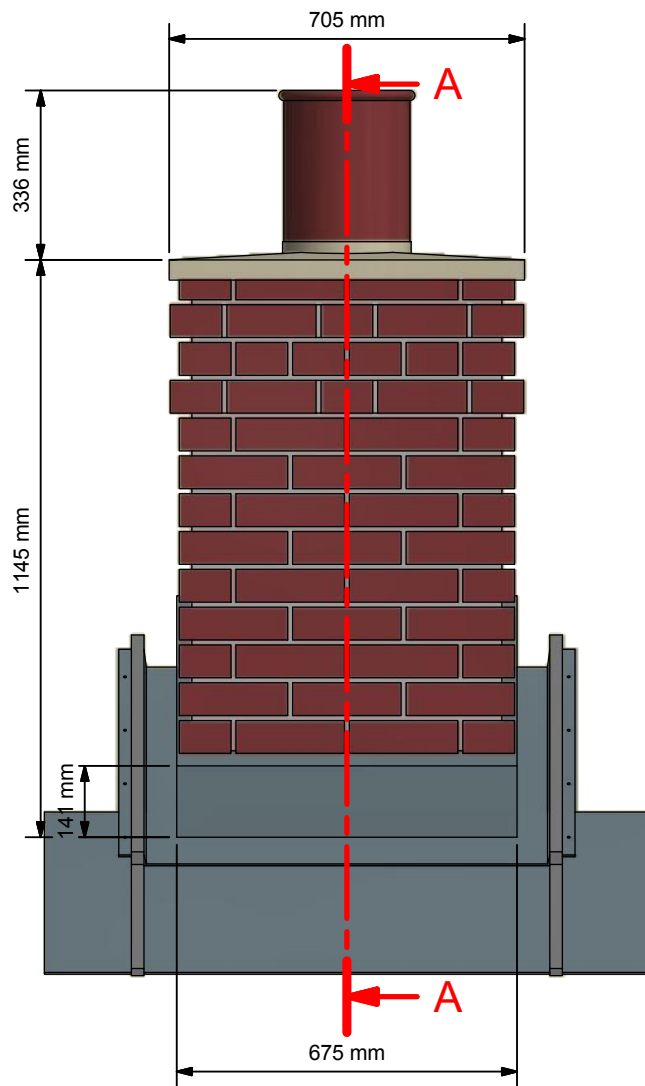
Typical Elevation ( 1:15 )
