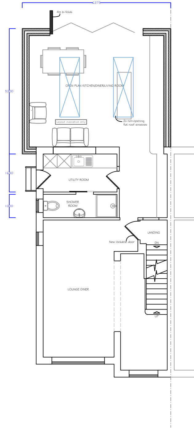
Proposed Plan 1:100 @ A3
