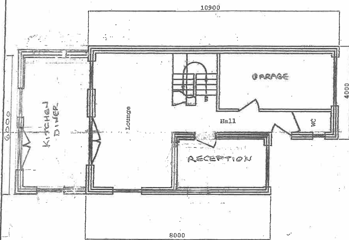
Ground Floor Plan (ORIGINAL)
