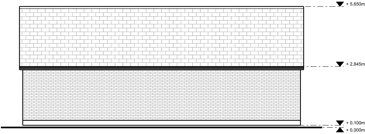
Rear Elevation
