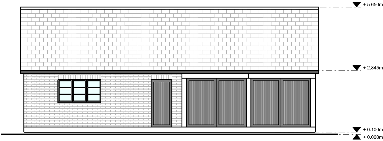
Front Elevation
