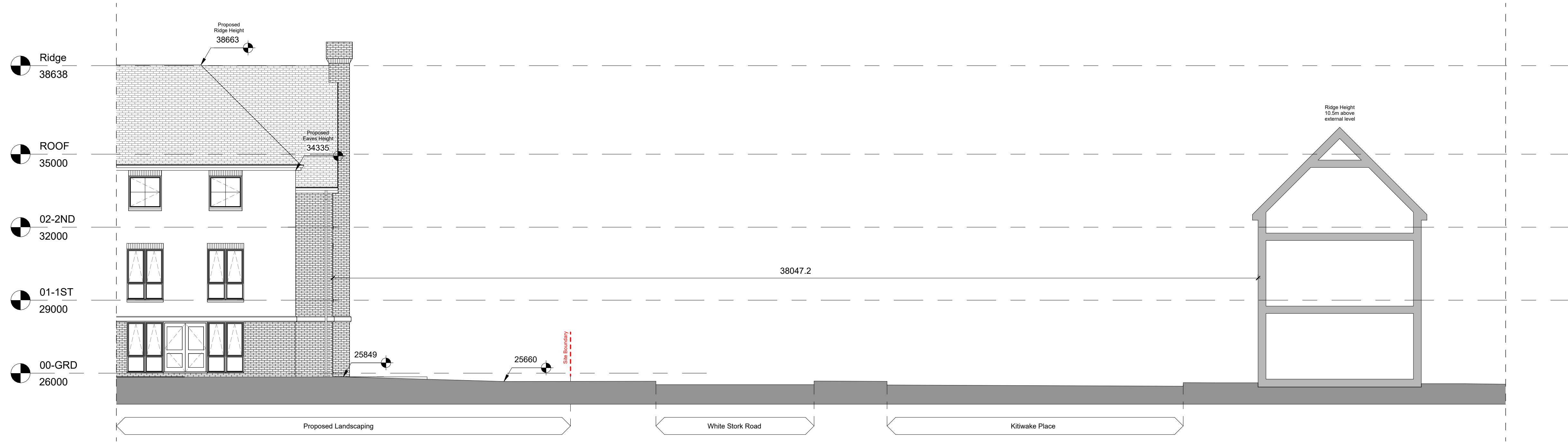
1 Proposed Site Section D-D 1 : 100
