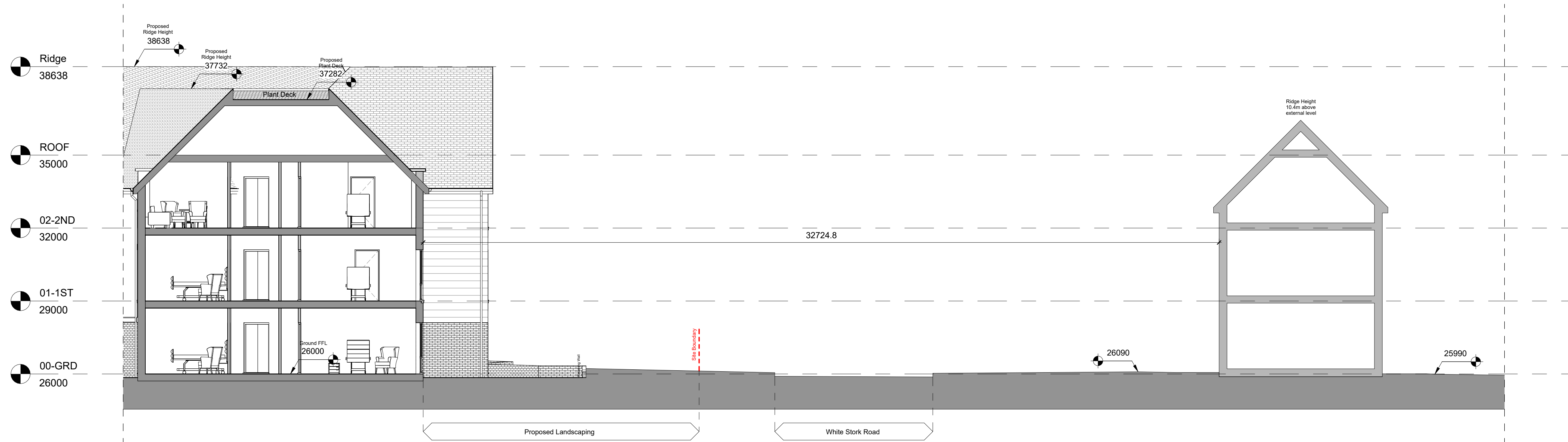
2 Proposed Site Section E-E 1 : 100
