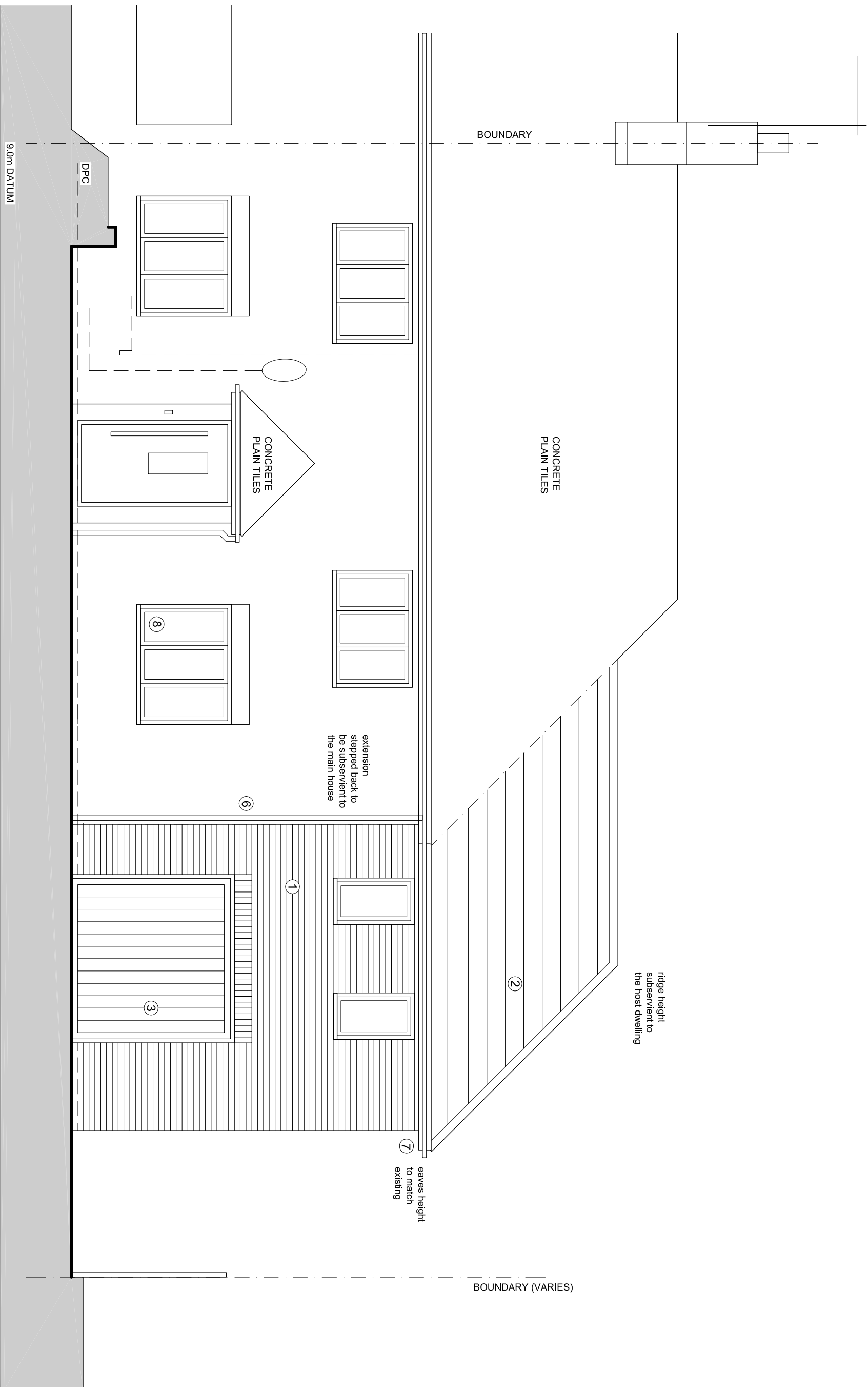
EAST ELEVATION
