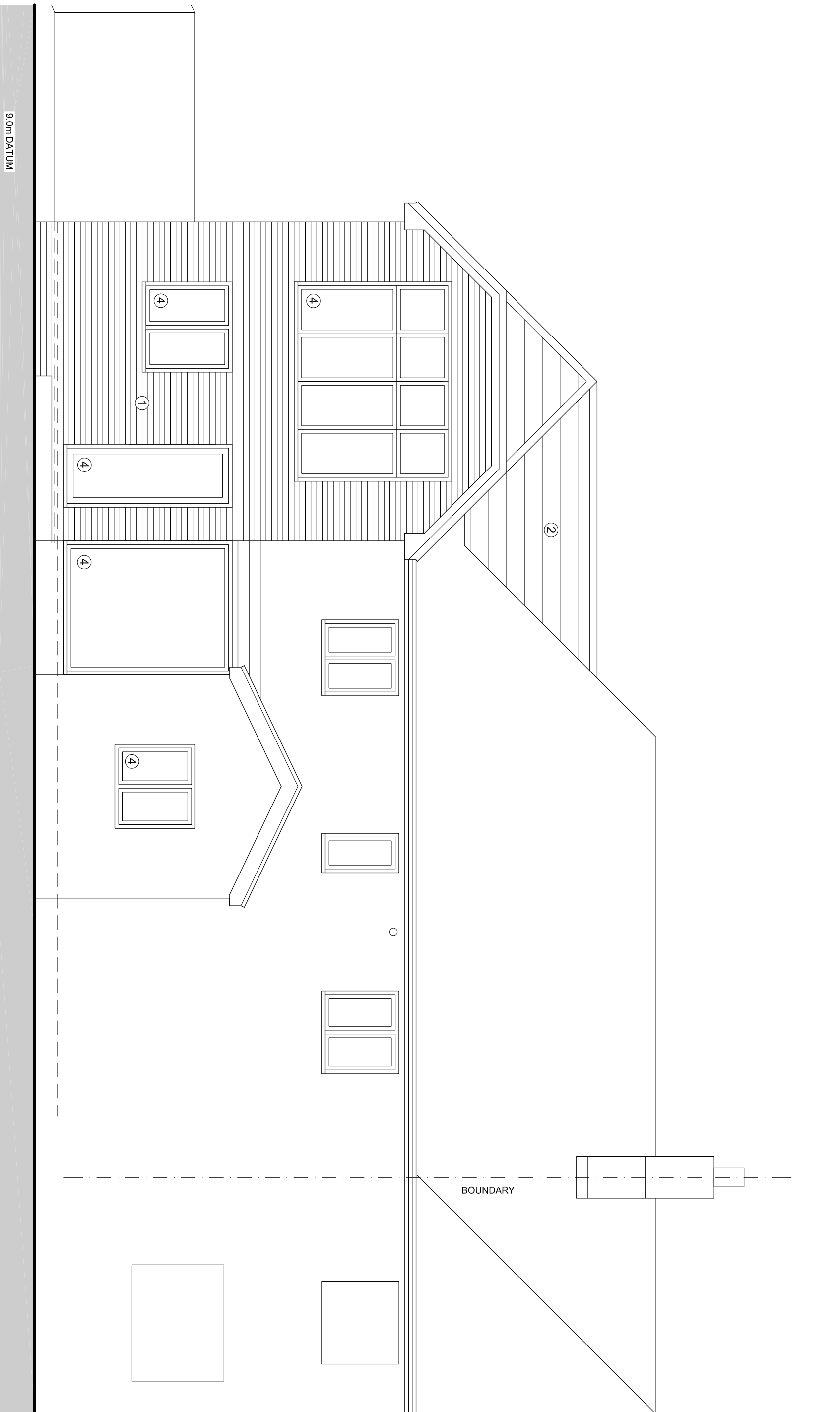
WEST ELEVATION
