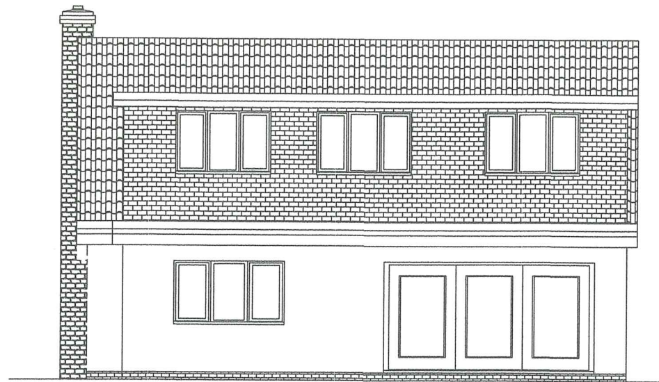
Rear Elevation
