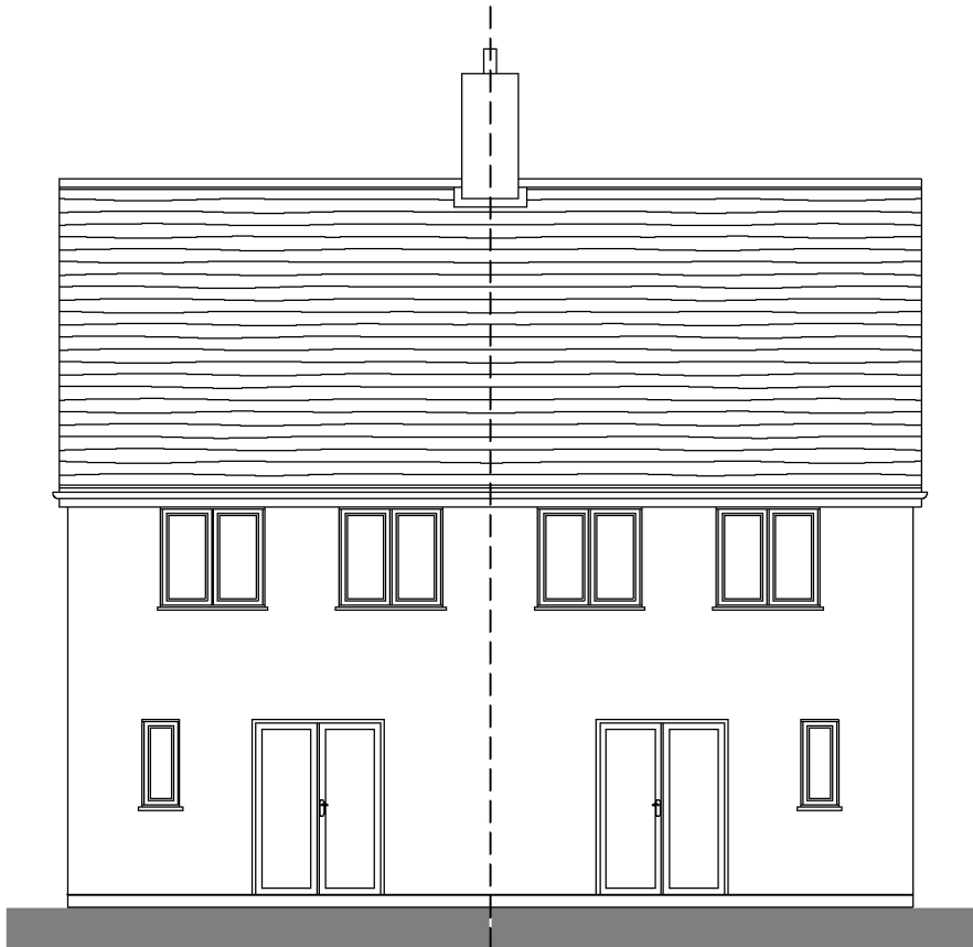
REAR ELEVATION
