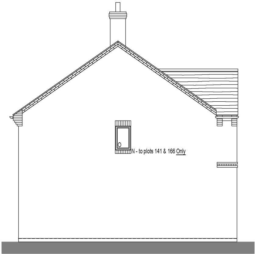
SIDE ELEVATION
