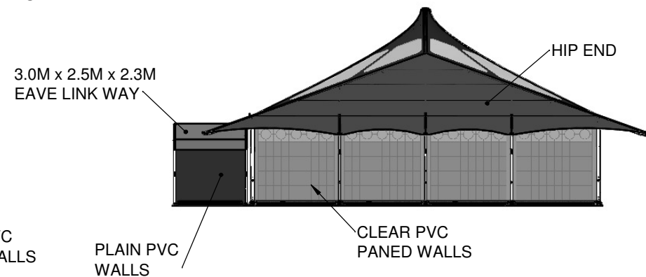
NORTH END ELEVATION
