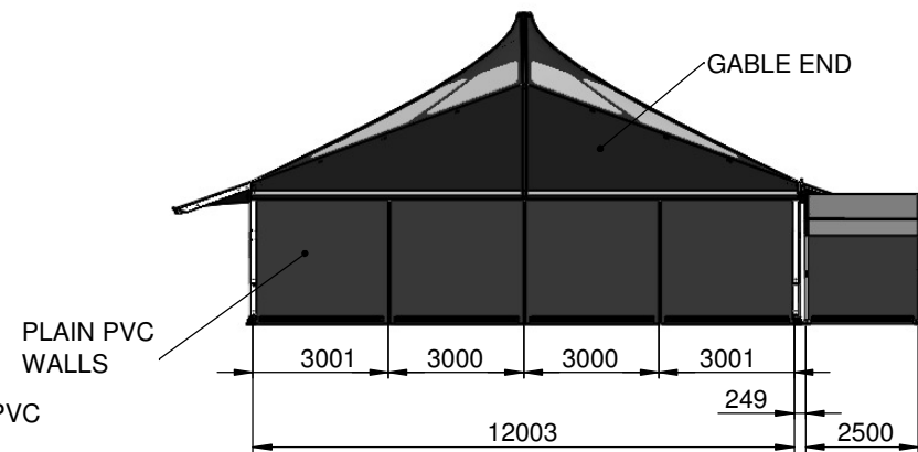
SOUTH END ELEVATION
