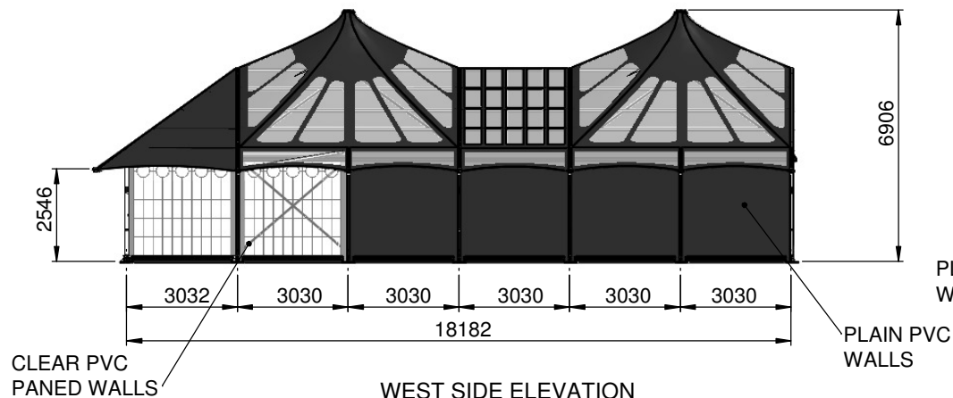
WEST SIDE ELEVATION
