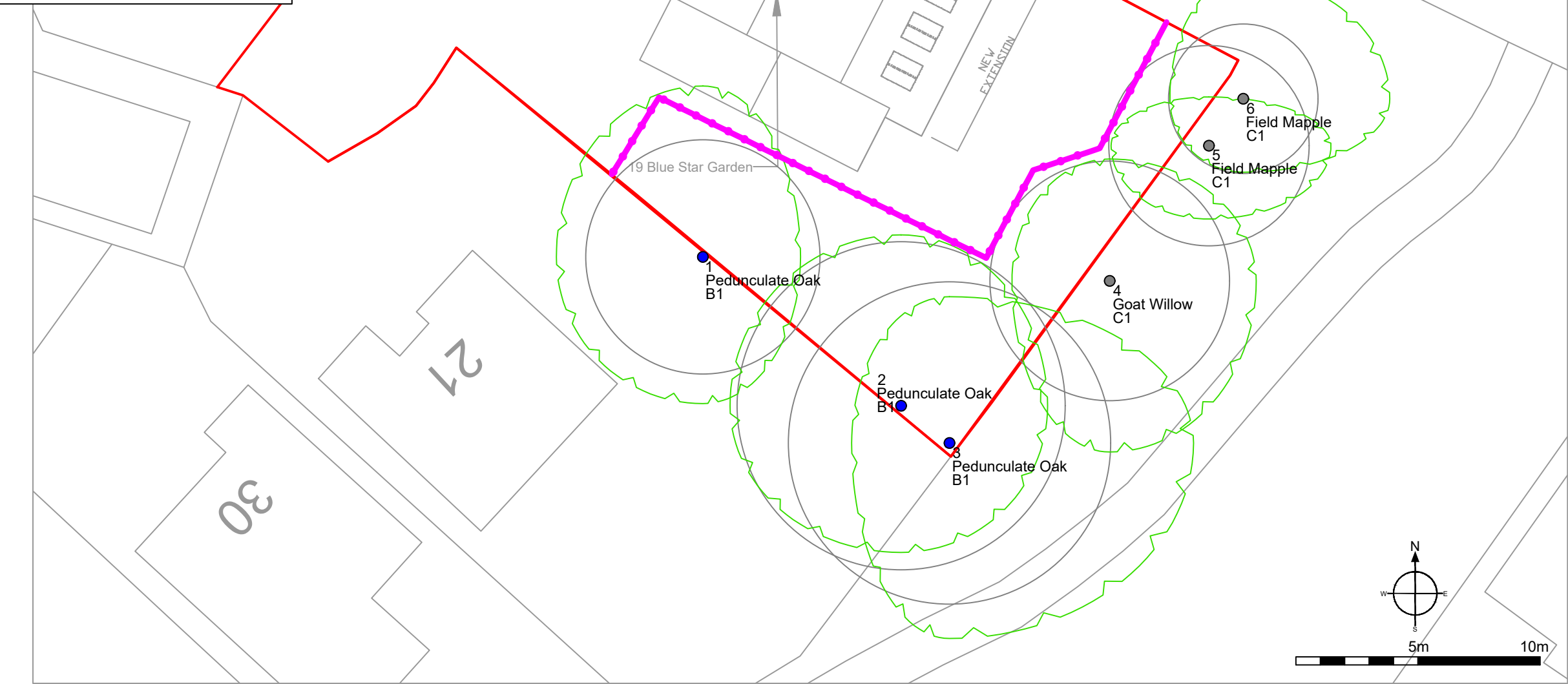
Sample tree protection from BS5837:2012
