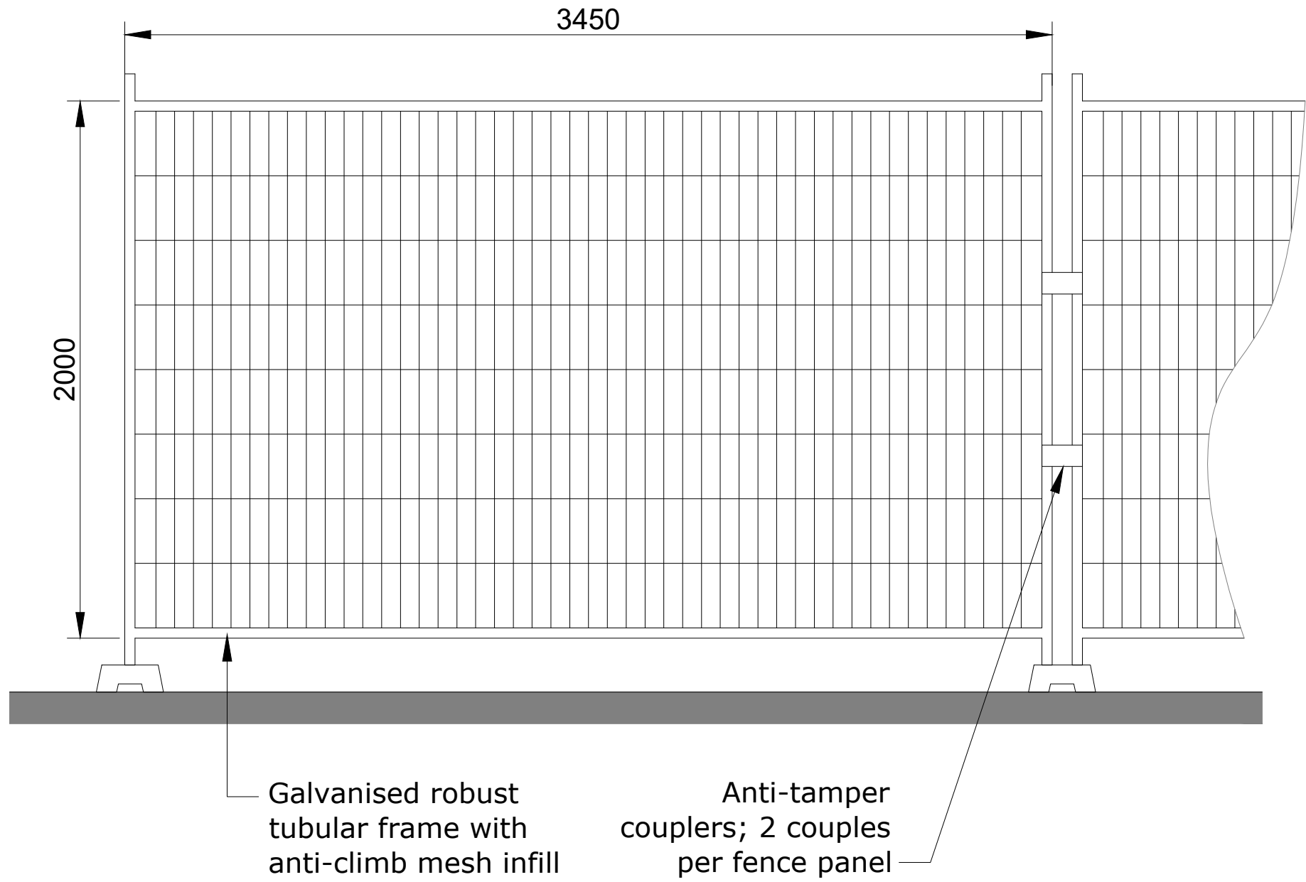
Typical Heras Tree Protection Fencing Detail 1:20
