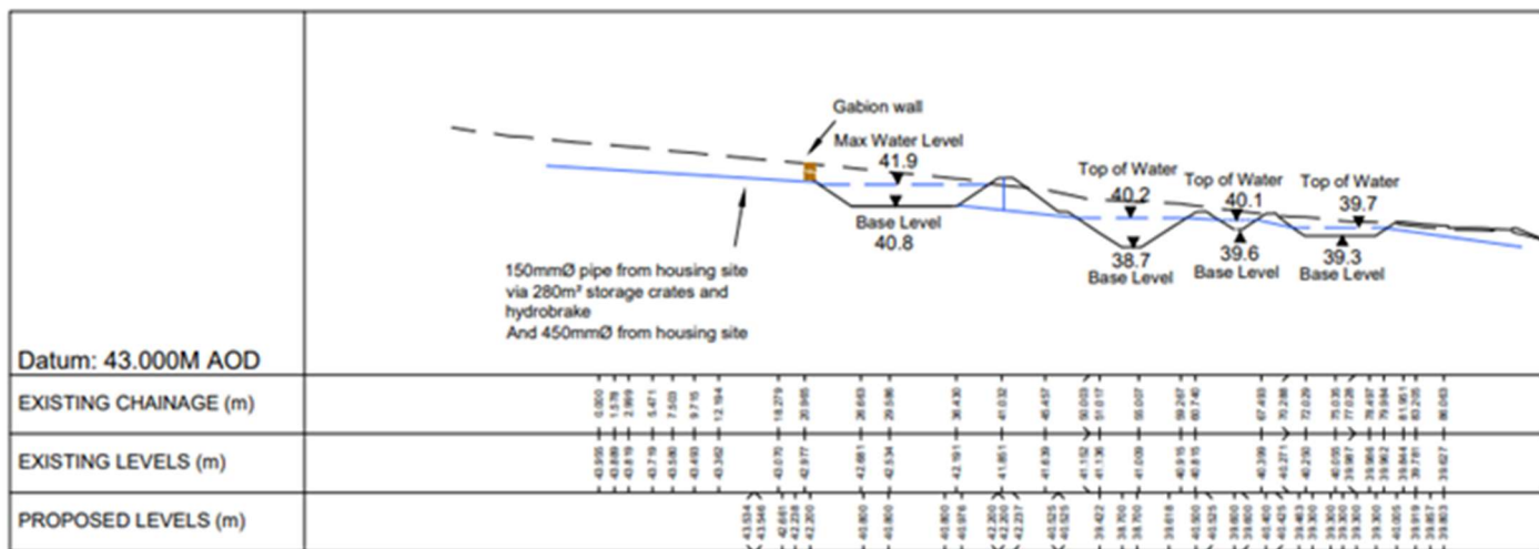
Section A-A Through Basins (2x vertical exaggeration)
