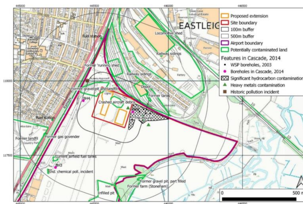
Figure 1: Summary of Potential Contamination (Source: Hannah Fraser report ref. 30691R2 Figure 2-5)
