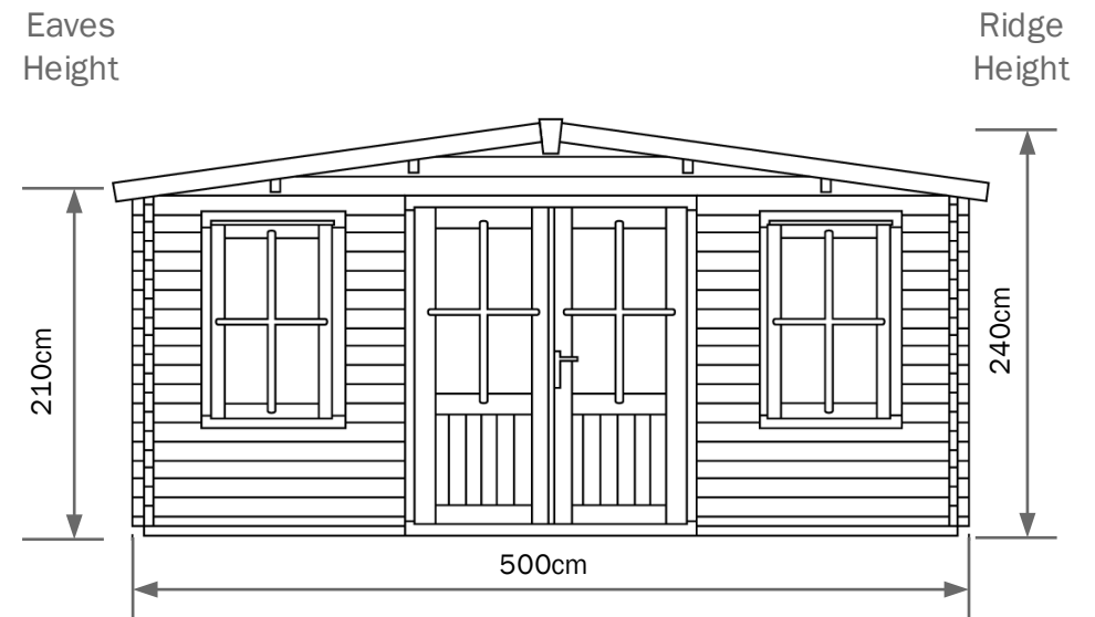
Front/Rear Elevation
