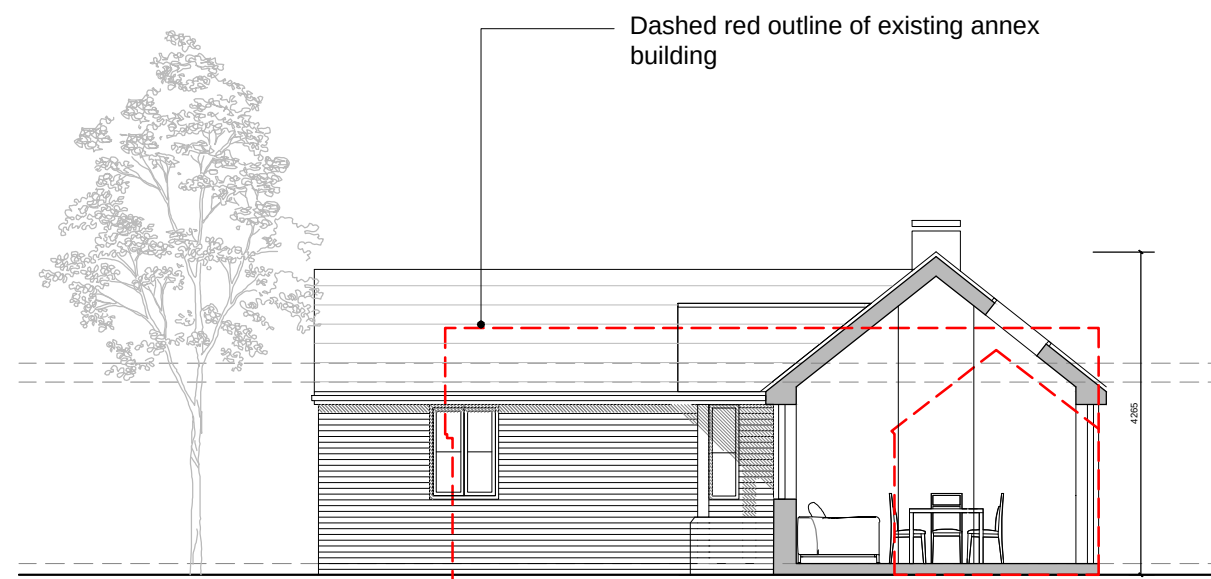
Typical Section as Proposed
