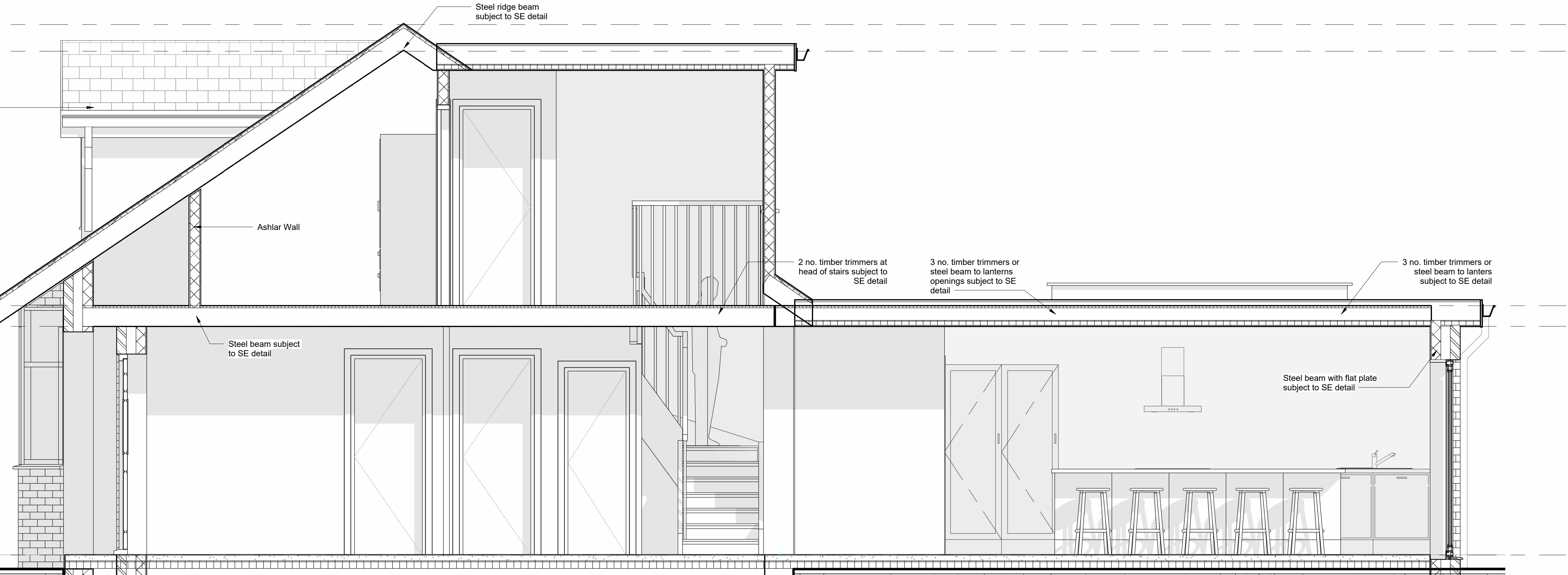
2 SECTION_B-B 1 : 25
