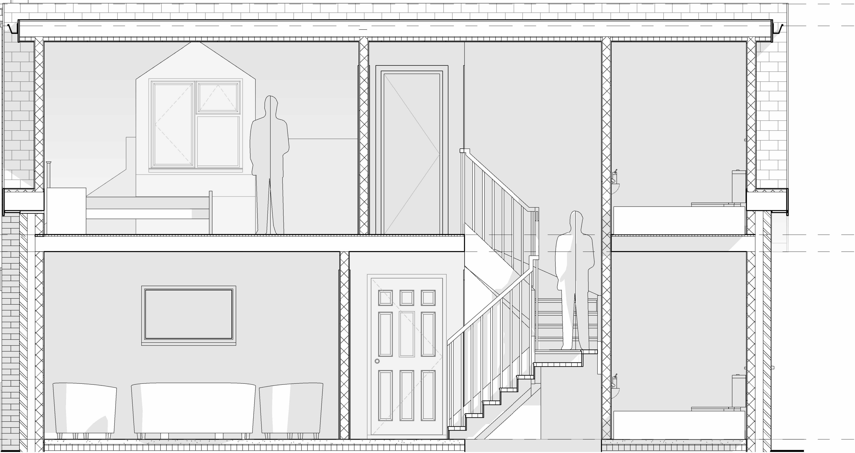
1 SECTION_A-A 1 : 25
