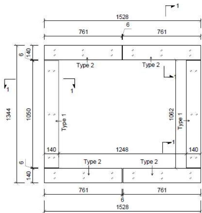
Elevation of Window Surround 1248x1050mm opening fixed to brickwork with 125mmx8mm s/s ribbed dowels Total required : 1no
