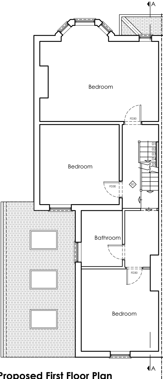
Proposed First Floor Plan Scale 1/100@A3
