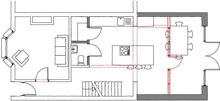
Ground Floor Plan Scale 1:50
