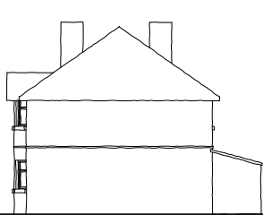
Side Elevation (North East) Scale 1:100
