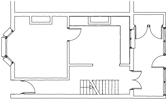
Ground Floor Plan Scale 1:50
