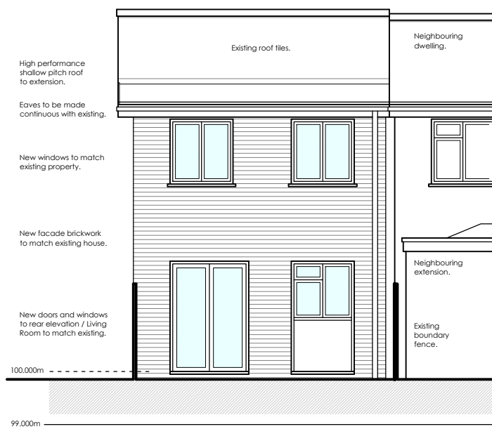
Proposed North-East Elevation 1:100
