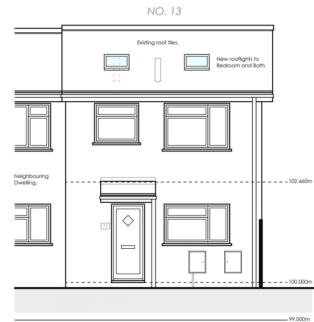
Proposed South-West Elevation 1:100
