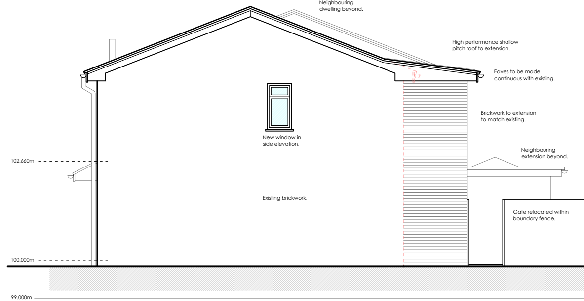
Proposed South-East Elevation 1:100
