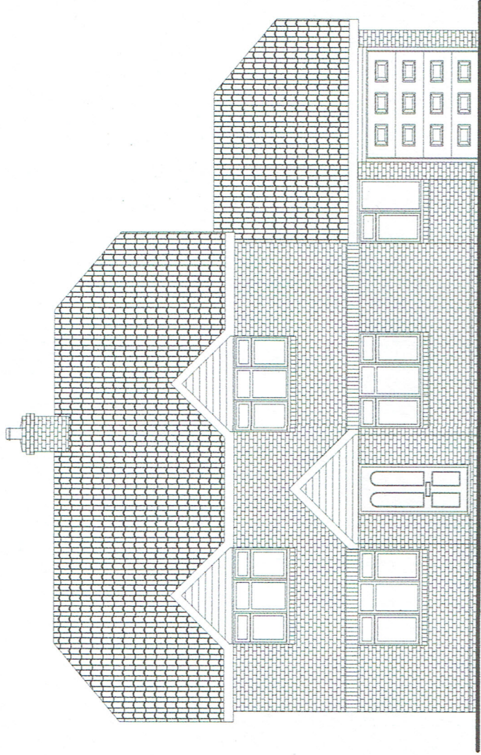
Front Elevation
