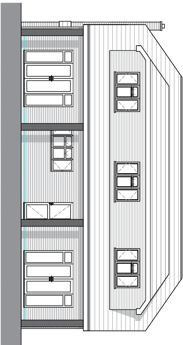
Proposed Rear Elevation 1:100 @ A3
