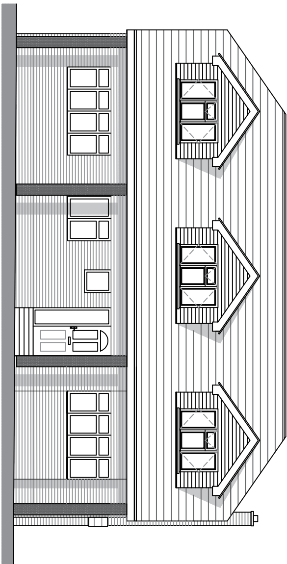
Proposed Front Elevation 1:100 @ A3
