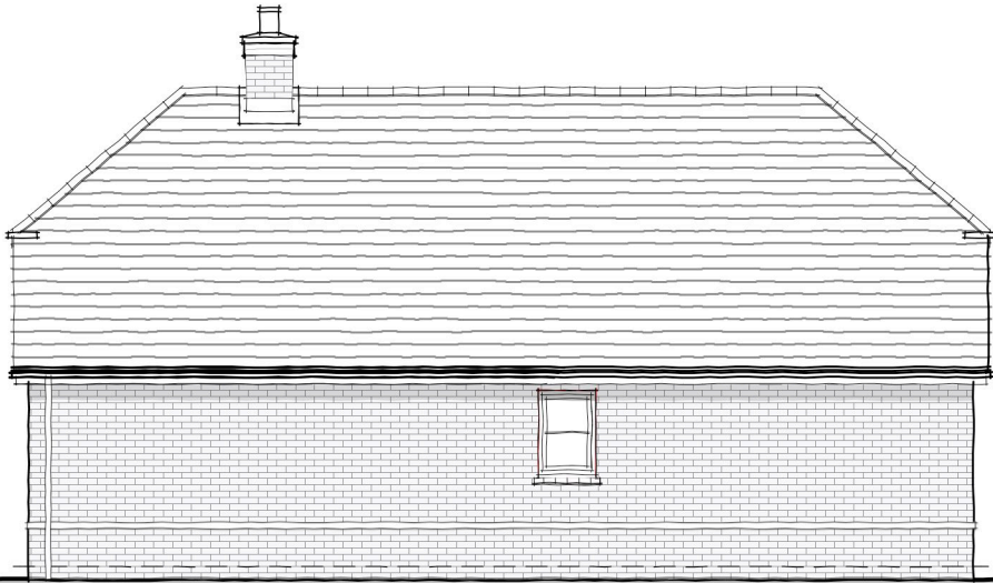
Rear Elevation
