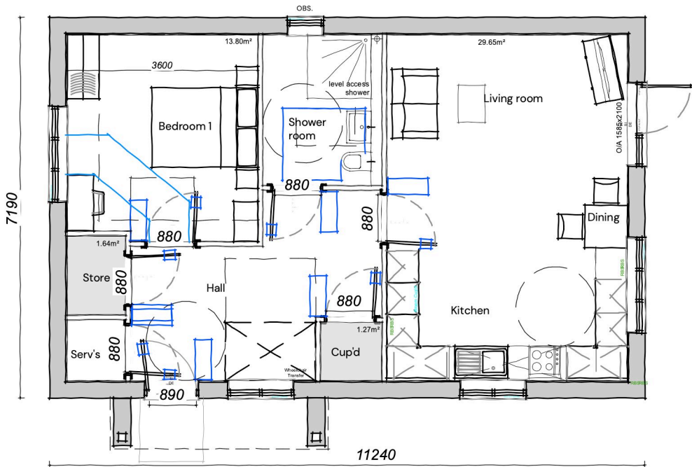
Floor Plan
