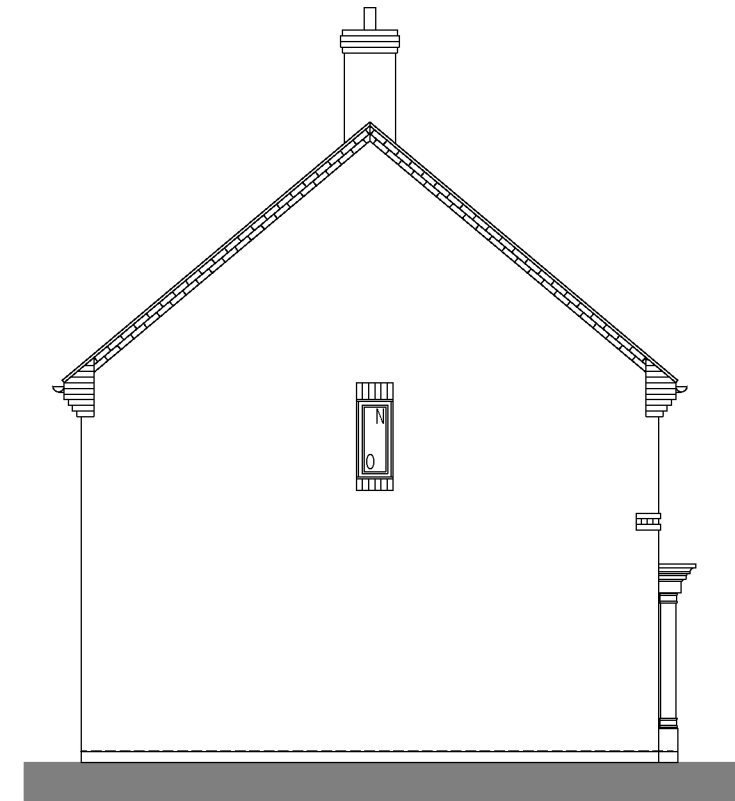
SIDE ELEVATION
