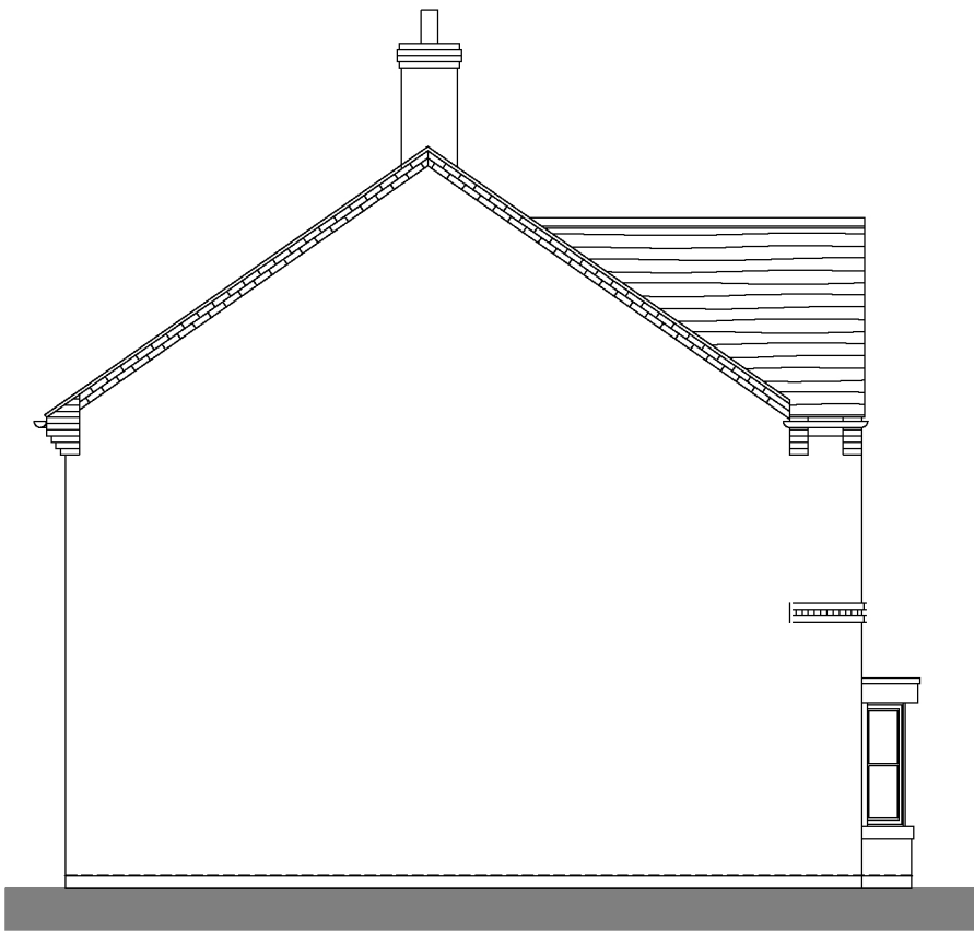
SIDE ELEVATION
