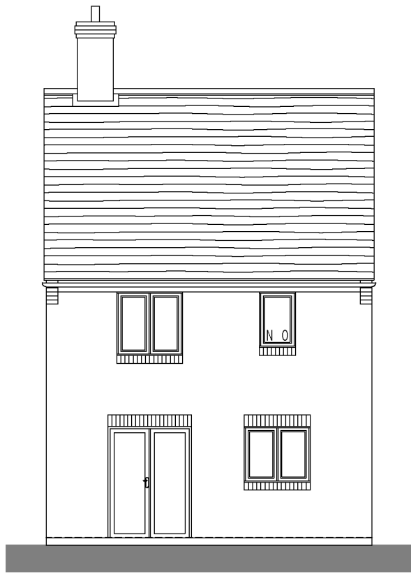
REAR ELEVATION
