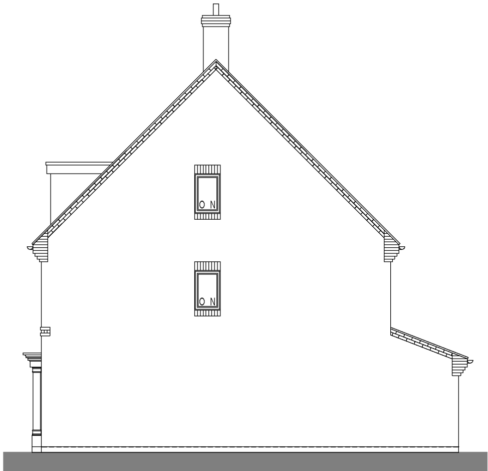
SIDE ELEVATION
