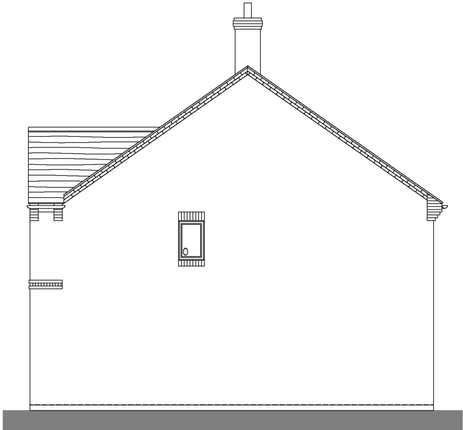
SIDE ELEVATION
