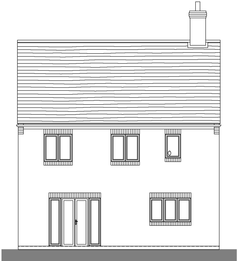
REAR ELEVATION
