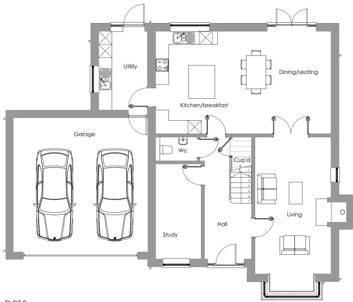
PLOT 9 As Proposed Ground Floor Plan 1:100
