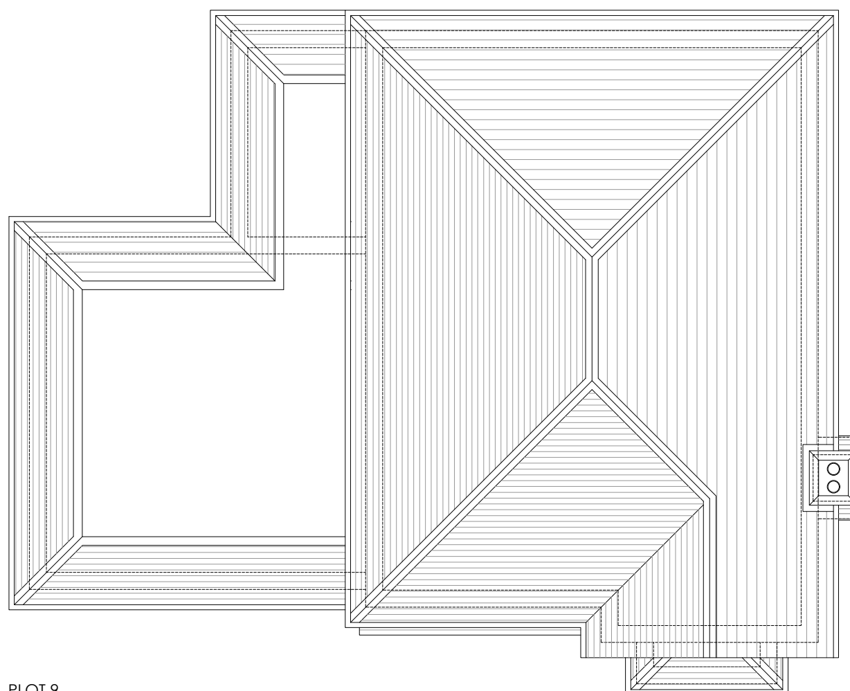
PLOT 9 As Proposed Roof Plan 1:100
