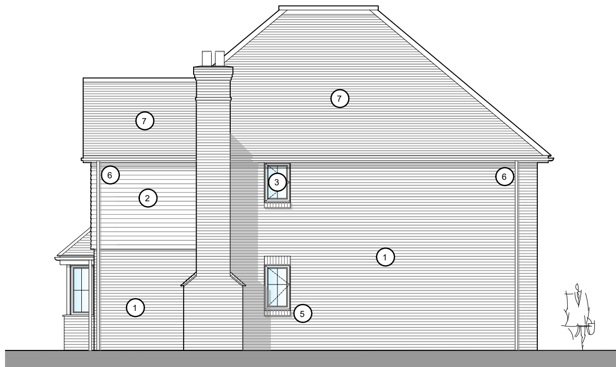
Plot 9 As Proposed South-East Elevation 1:100
