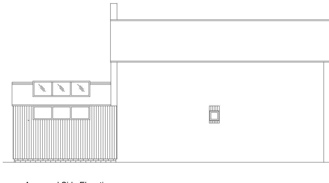
Approved Side Elevation Prepared by CFW Architects
