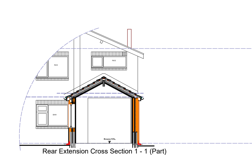
Rear Extension Cross Section 1 - 1 (Part)
