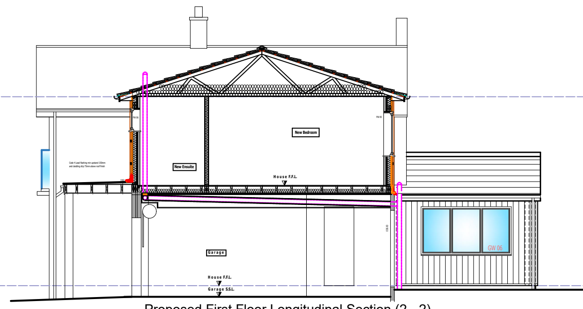
Proposed First Floor Longitudinal Section (2 - 2)
