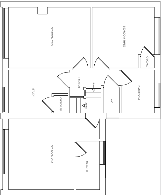
Proposed First Floor Plan 1:100 @ A3
