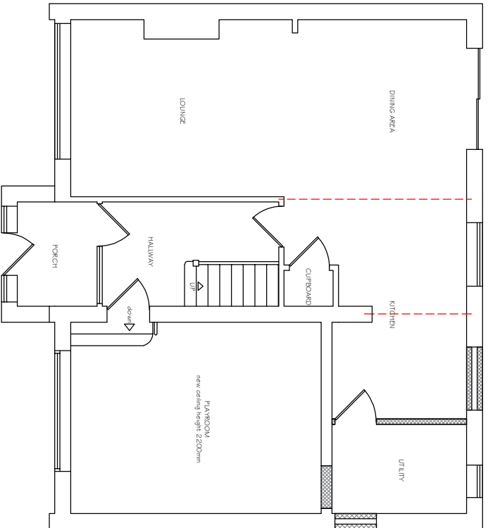
Proposed Ground Floor Plan 1:100 @ A3
