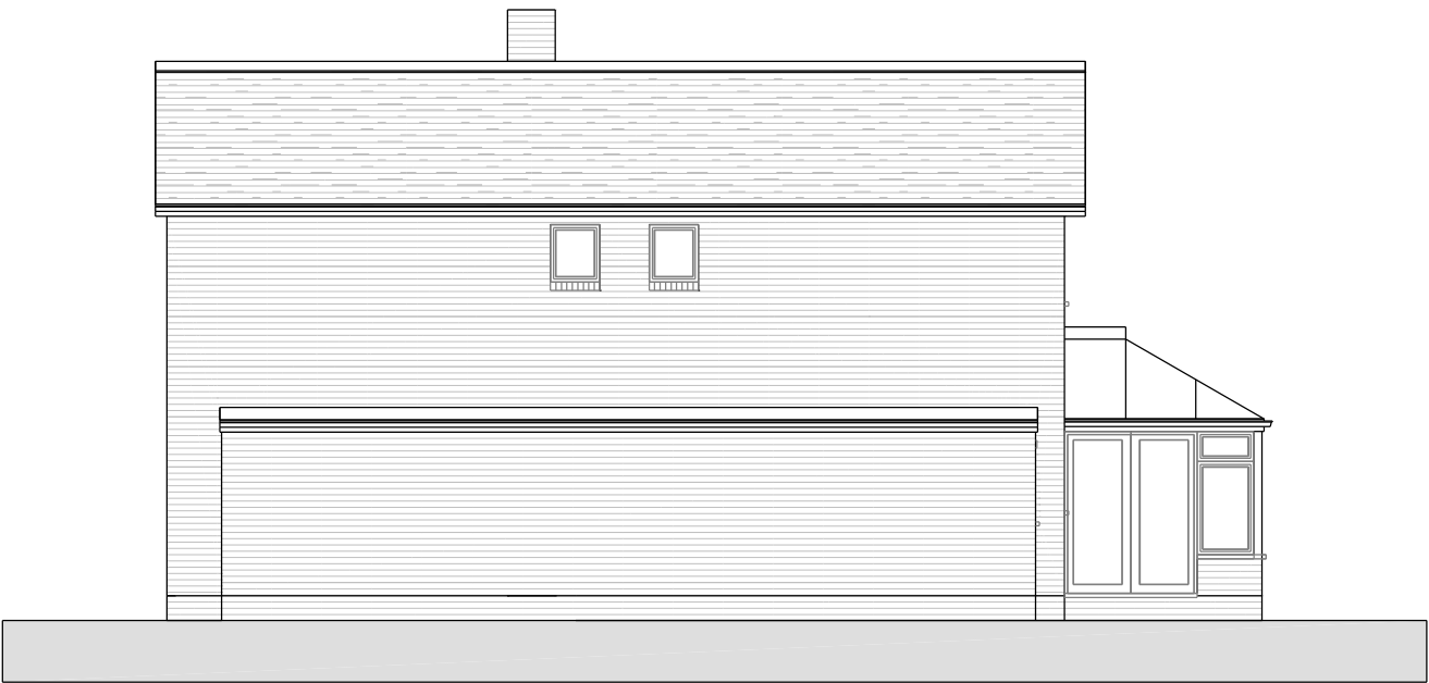
EXISTING SIDE ELEVATION - NORTH EAST Scale 1:100 @ A3
