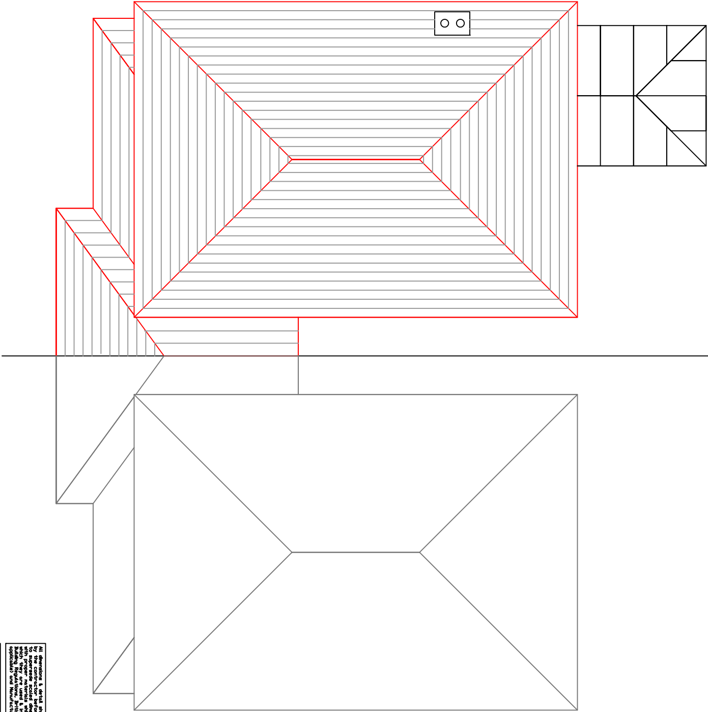
EXISTING ROOF
