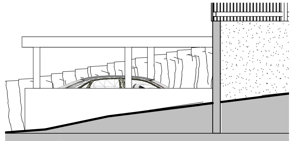
2 Garage North Elevation 1 : 50
