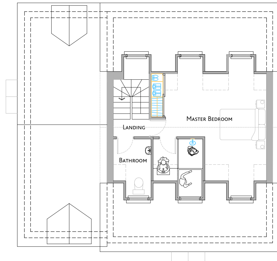
PROPOSED ATTIC CONVERSION
