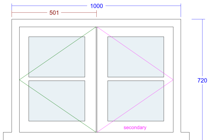
4. Conventional Cottage Window (Kitchen W3 )
