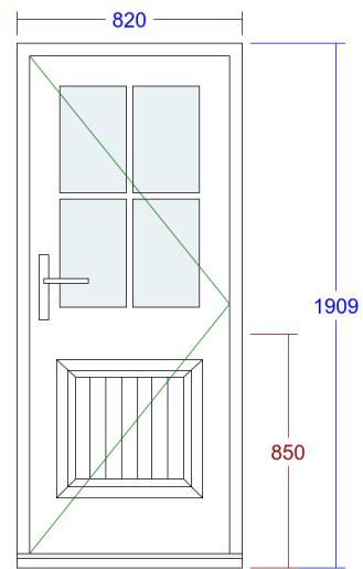
13. Entrance Door (Back door )
