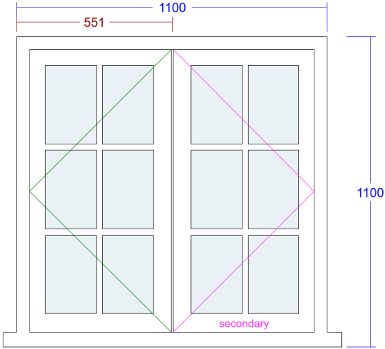
8. Conventional Cottage Window (Rear bed W1 )
