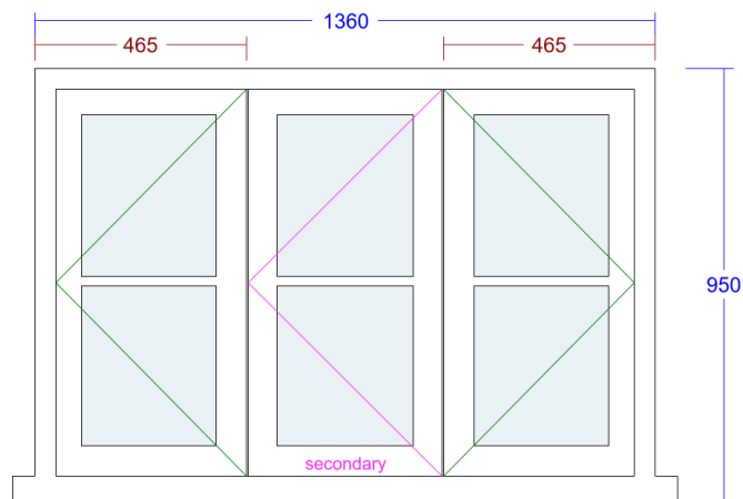
5. Conventional Cottage Window (Living room rear )
