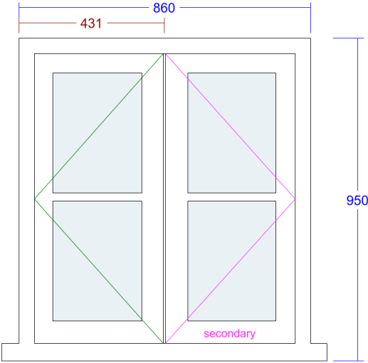
9. Conventional Cottage Window (Rear bed W2 )
