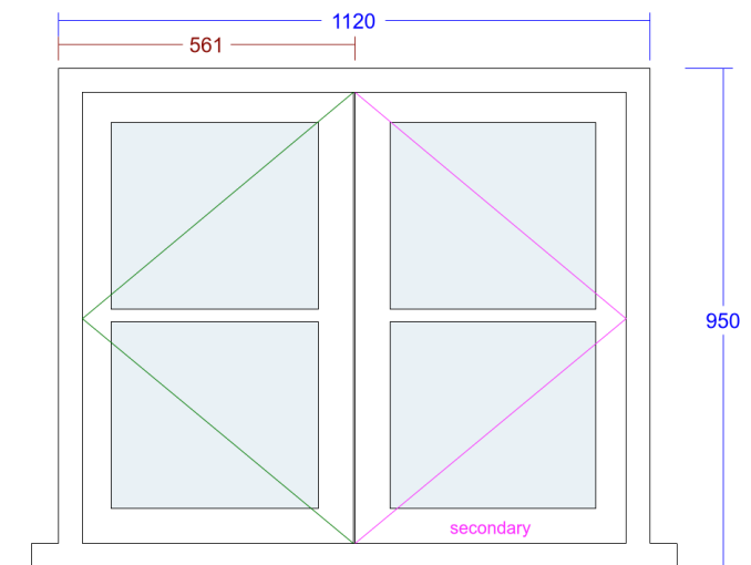
6. Conventional Cottage Window (Living room side )
