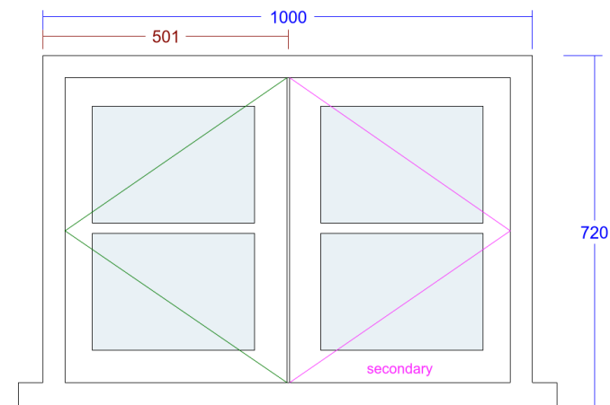
3. Conventional Cottage Window (Kitchen W2 )
