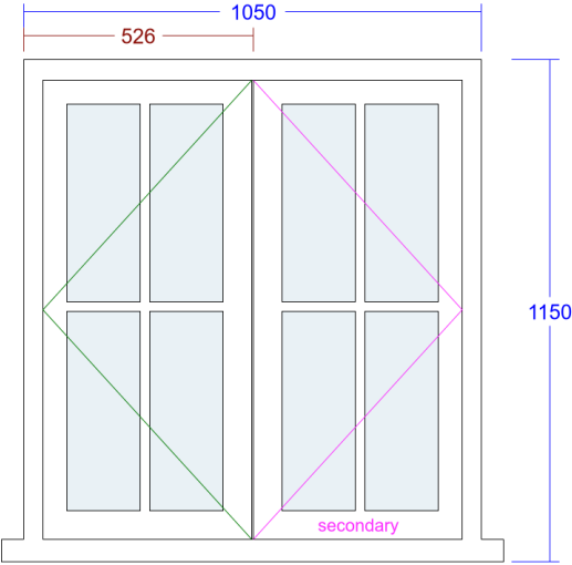
10. Conventional Cottage Window (Study/bedroom )
