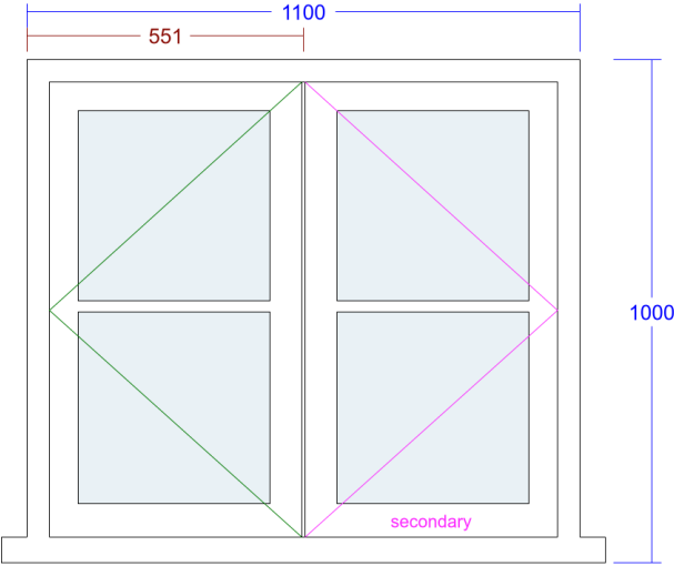
7. Conventional Cottage Window (Attic bedroom )
