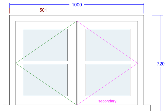
2. Conventional Cottage Window (Kitchen W1 )
