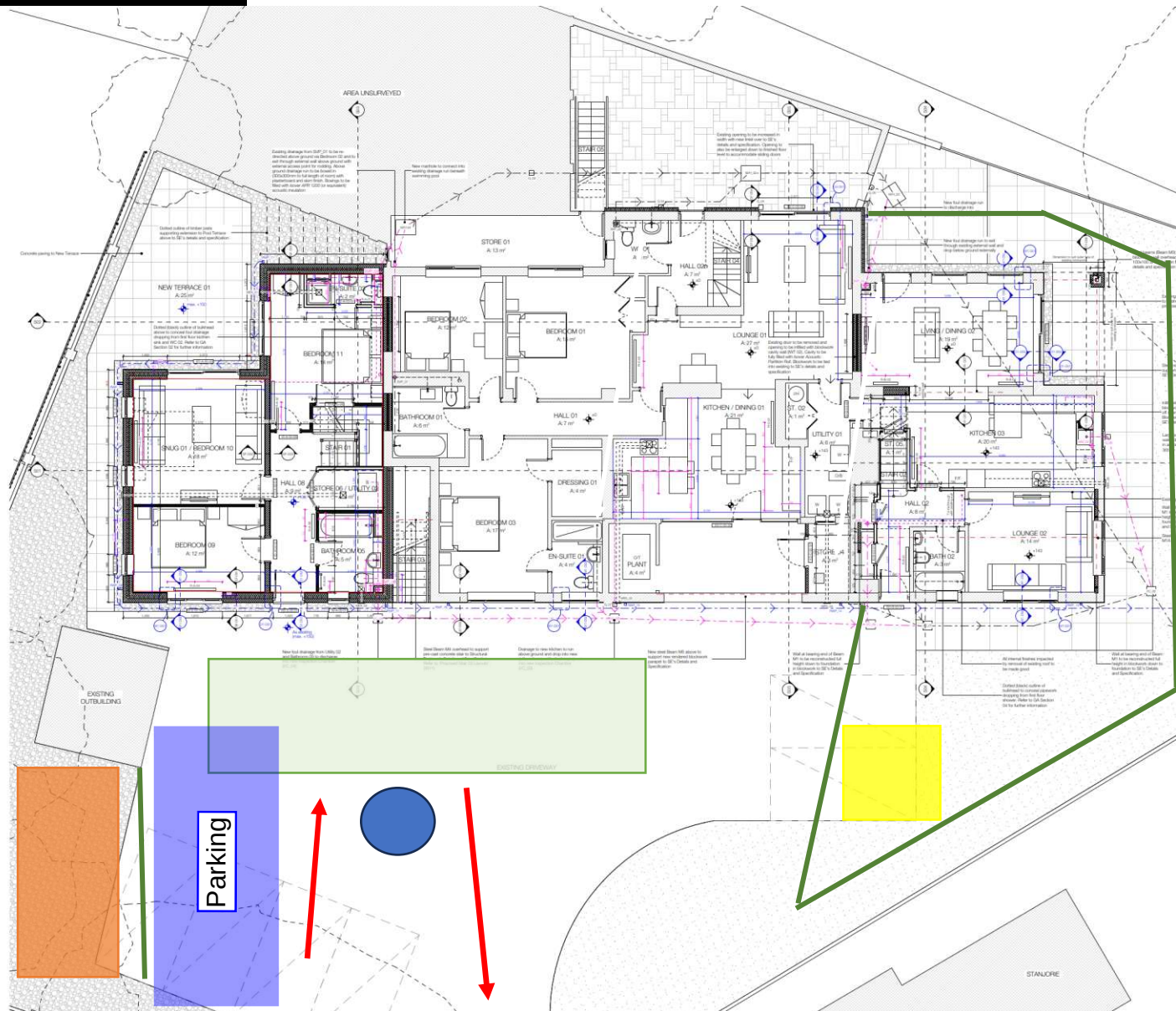
Brooklands, Botley - Site Logistics Plan
