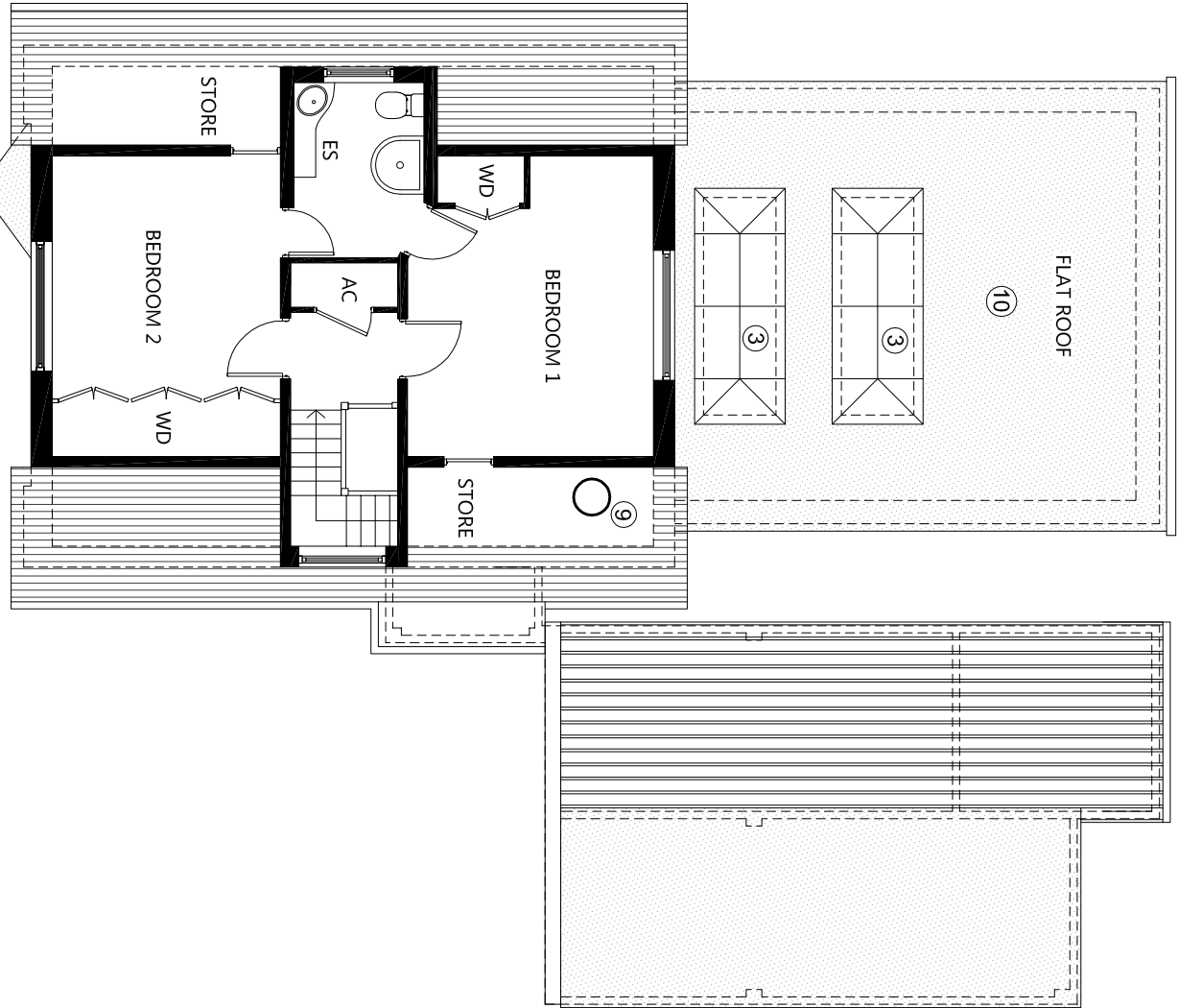
PROPOSED FIRST FLOOR / ROOF PLAN @ 1:100 SCALE
