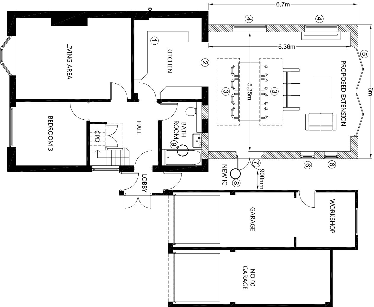
PROPOSED GROUND FLOOR PLAN @ 1:100 SCALE
