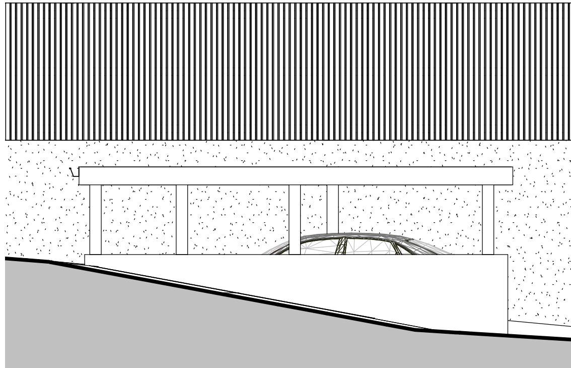
3 Garage South Elevation 1 : 50
