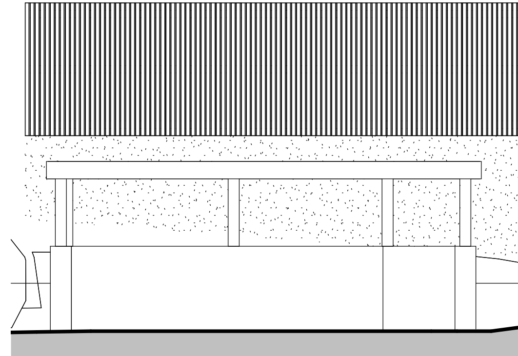
1 Garage East Elevation 1 : 50
